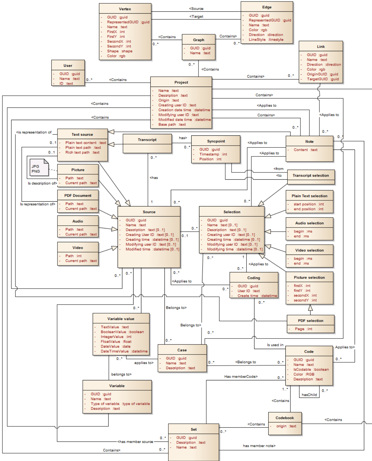
Figure 2. Overall data model
