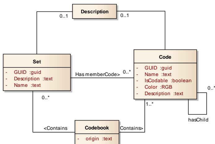
Figure 3. Data model for code book exchanges
